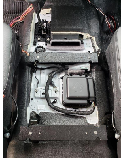
Step 2 - install cross braces
